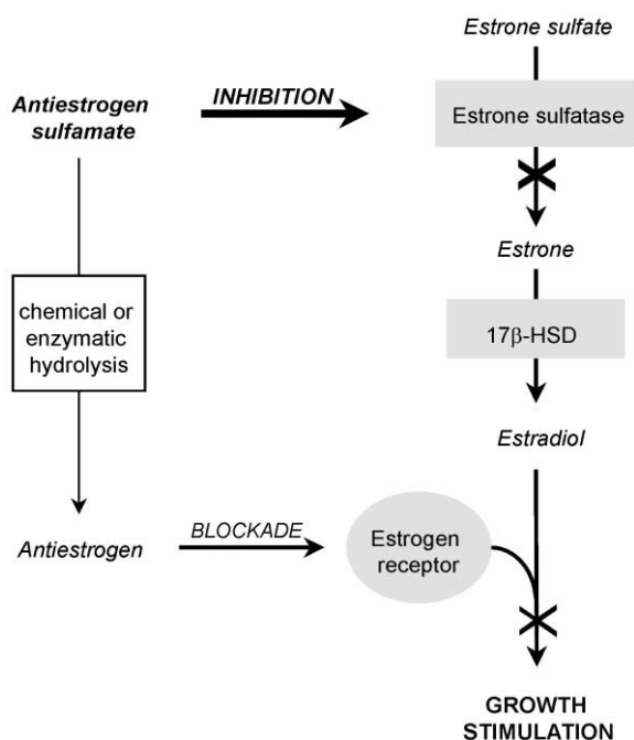
Figure 2. Stimulation of breast cancer growth by estrone sulfate: points of intervention by antiestrogen-based steroid sulfatase inhibitors.
