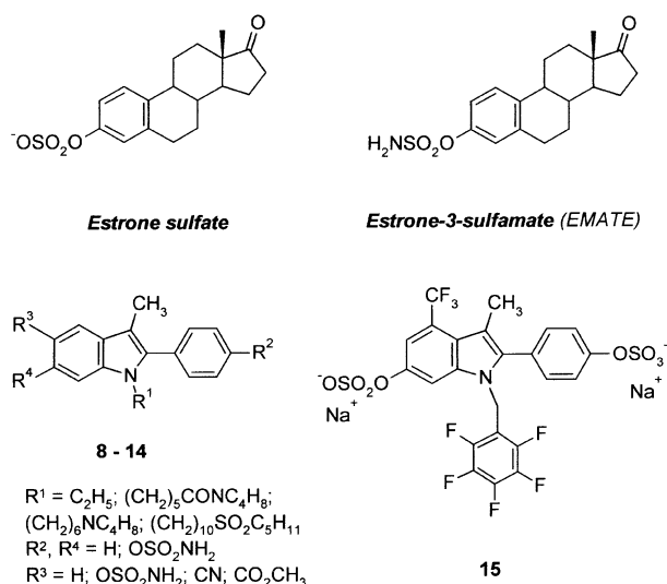
Figure 1. Chemical structures of estrone sulfate, estrone-3-sulfamate (EMATE) and 2-phenylindole-based inhibitors of steroid sulfatase.
